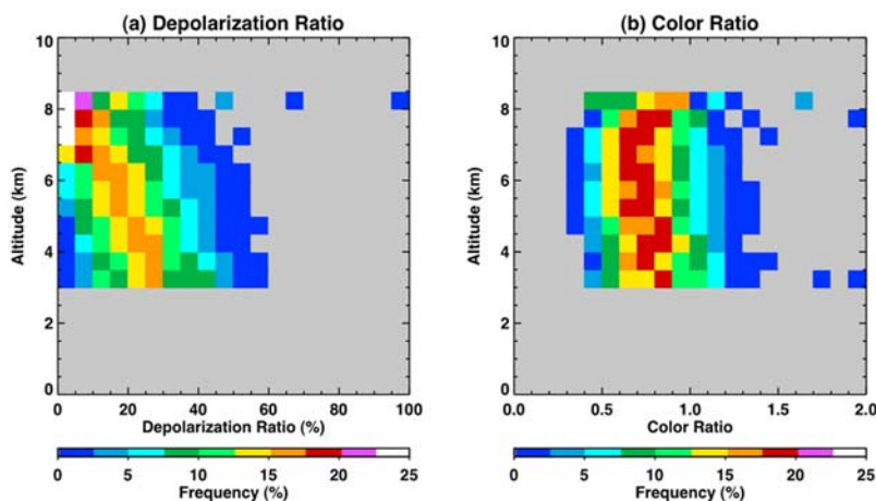
Figure 3. Frequency distribution of (a) the depolarization ratio and (b) the color ratio as functions of altitude for the 10 selected cases.
