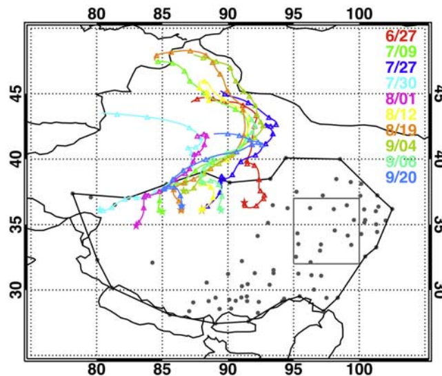
Figure 4. Four-day back trajectories of air parcels climbing upon the Tibet Plateau for the 10 cases listed in Table 1. The gray dots represent surface observation station.
