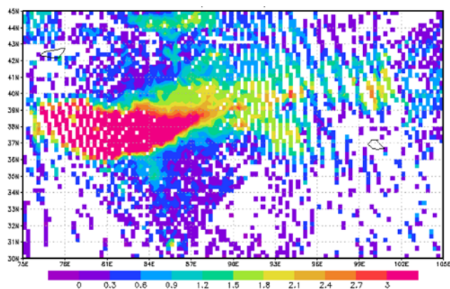
Figure 2. Aura OMI aerosol index over Taklamakan Desert and Tibet Plateau on 28 July 2006.
