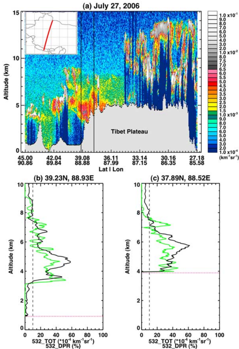
Figure 1. (a) The altitude-orbit cross-section of total attenuated backscattering intensity over Taklamkan-Tibet Plateau. (b) The vertical profiles of total 532 nm attenuated backscattering intensity (black curve) and depolarization ratio (green curve) about 20 GMT on 27 July 2006 at 39.23°N, 88.93°E. (c) Same as in Figure 1b but for 37.89°N, 88.52°E.
